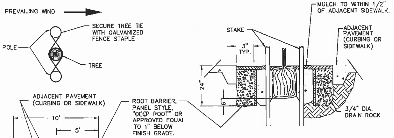
TREE ROOT BARRIER DETAIL NOT TO SCALE
